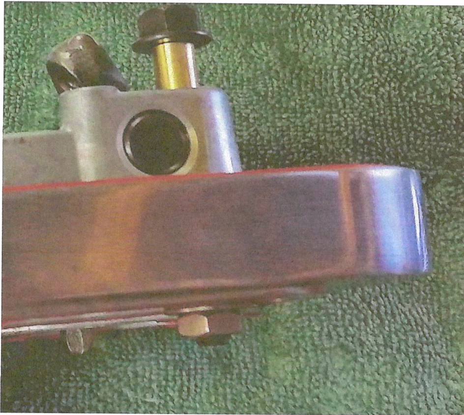
This photo shows the Rocker Locker being pressed into the Rocker Cover Inner by slowly turning the bolt with a wrench, while holding the nut stationary with another wrench.
